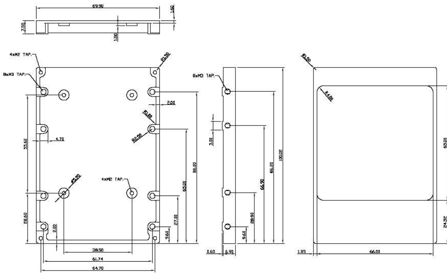
Figure 2-1. 2.5" SSD Dimensions
