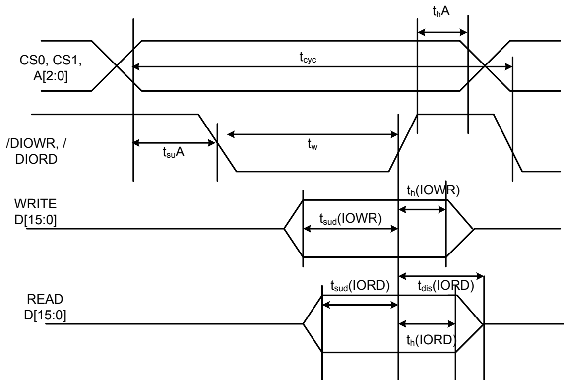
Figure 3-3. Register Transfer To/From Device
