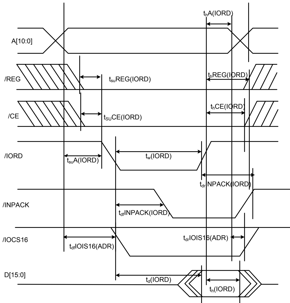
Figure 3-2. I/O Read Timing Diagram
