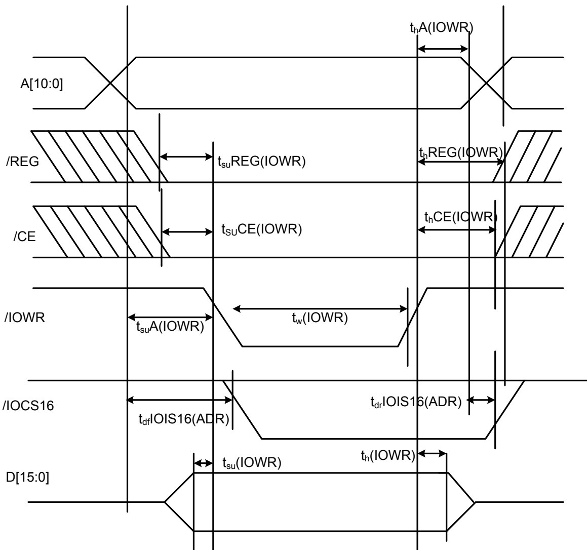
Figure 3-2. I/O Write Timing Diagram
