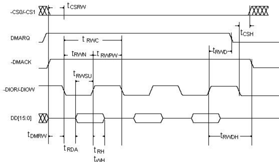
Figure 3-4. DMA Transfer To/From Device
